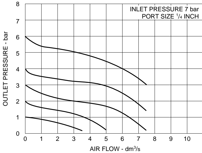
FLOW CHARACTERISTICS
