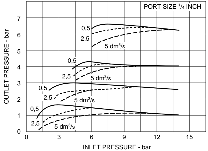
REGULATION CHARACTERISTICS
